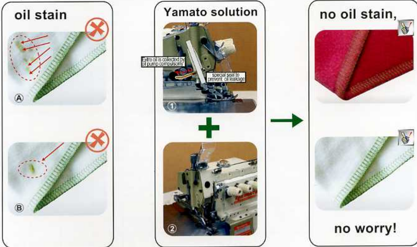
Pic ① pump collecting extra oil mechanism (patent pending)
